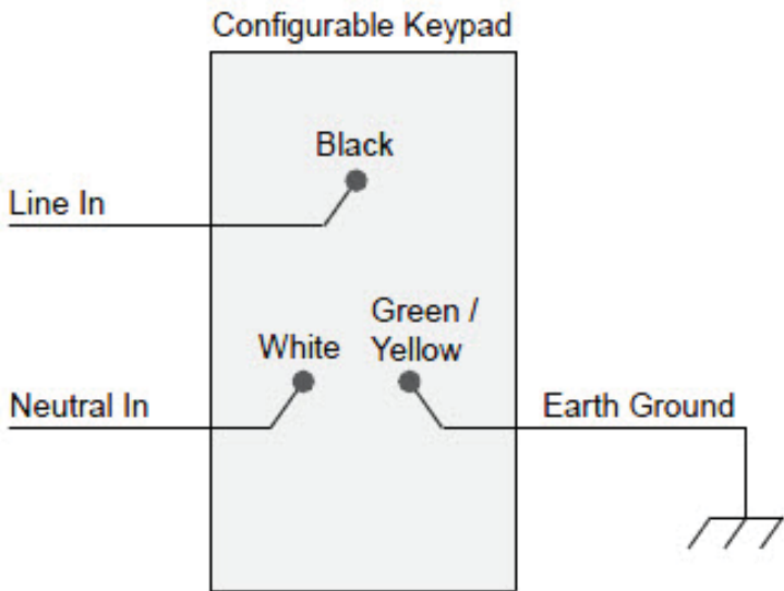
Figure 2. Keypad Wiring
