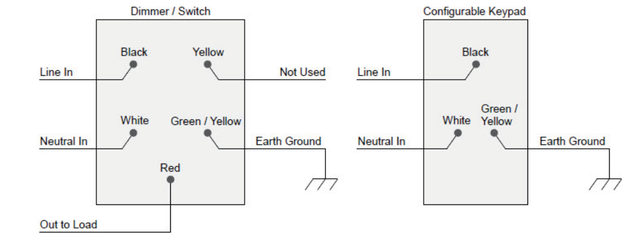
Figure 8. Multiple Device Location Using Configurable Keypad, Neutral Required
