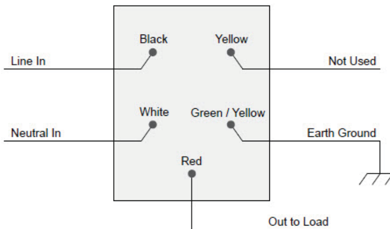
Figure 4. Single Device Location, With Neutral Connection
