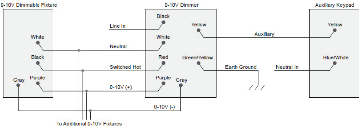
Figure 4. Multiple Device Location Using Auxiliary Keypad, With Neutral Connection
