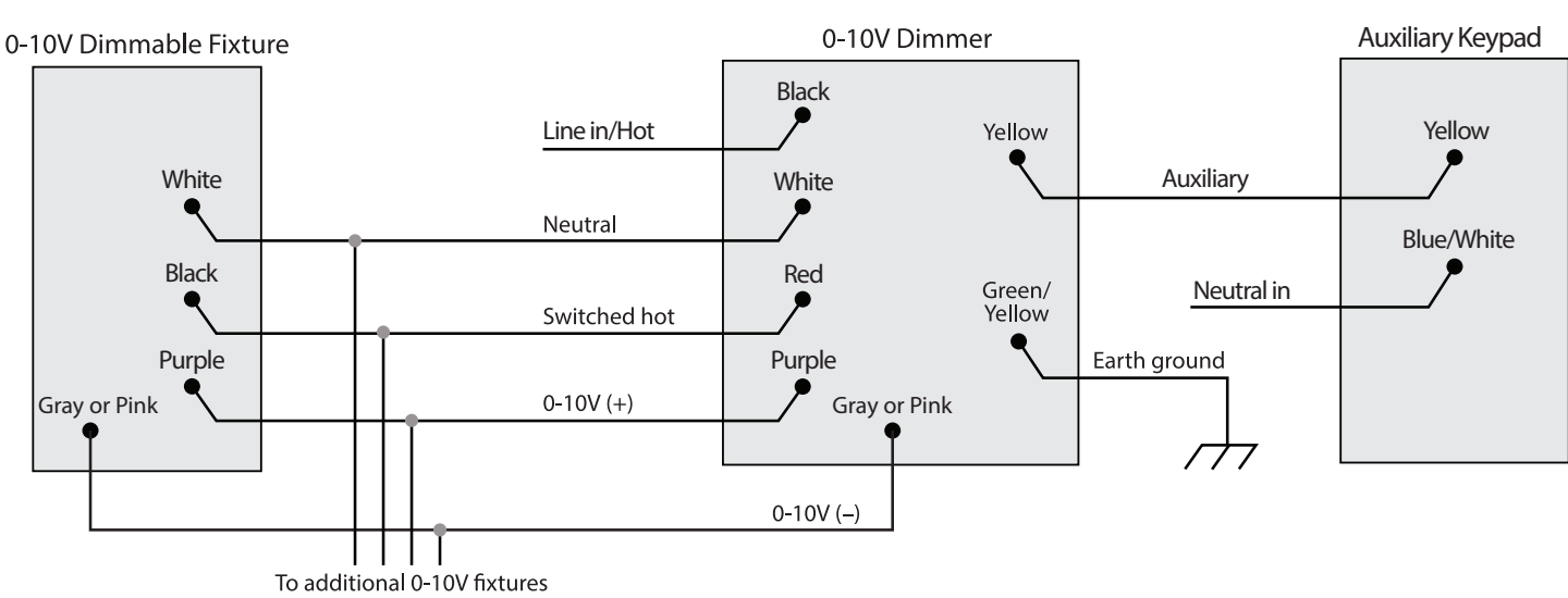
Figure 4. Multiple device location using Auxiliary Keypad, with neutral connection
