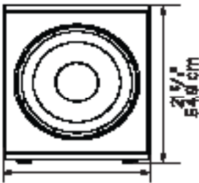
18 1/2" 47 cm (Front)
