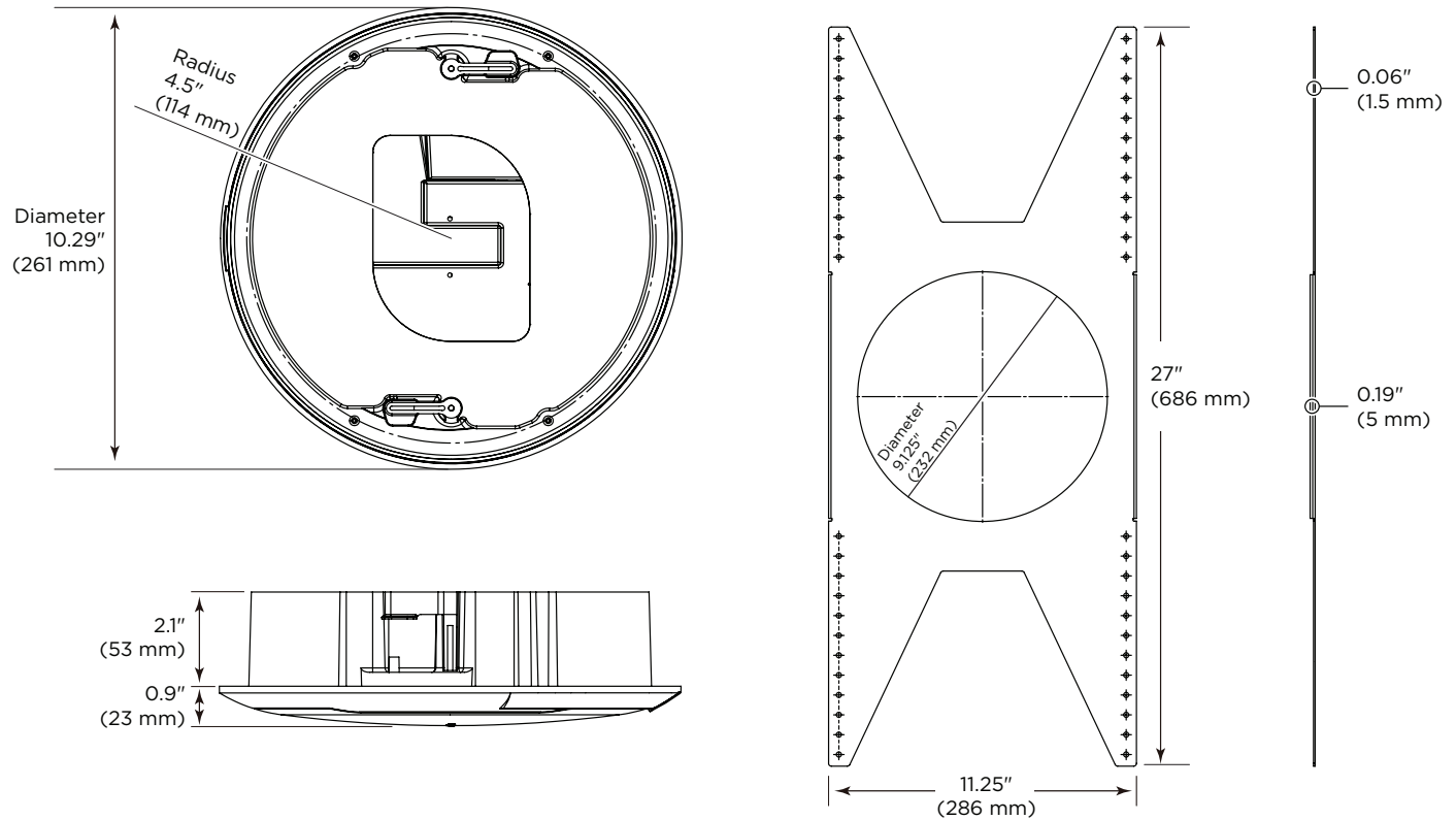
WK-2-C bracket dimensions
