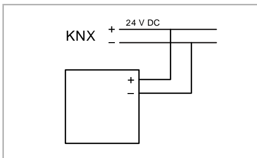
Fig. 6: Connection of bus coupler
