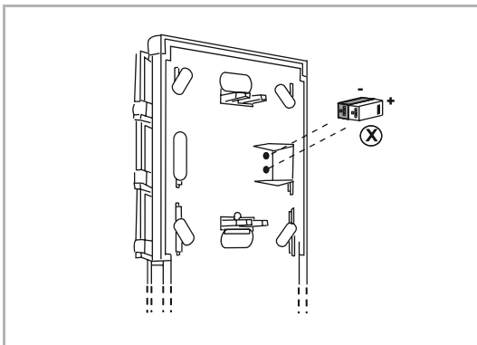
Fig. 9: Mounting the bus terminals
