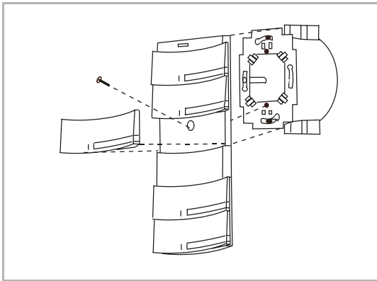
Fig. 10: Mounting the device
