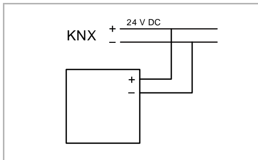
Fig. 12: Connection of bus coupler
