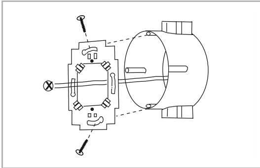
Fig. 8: Mounting the support ring
