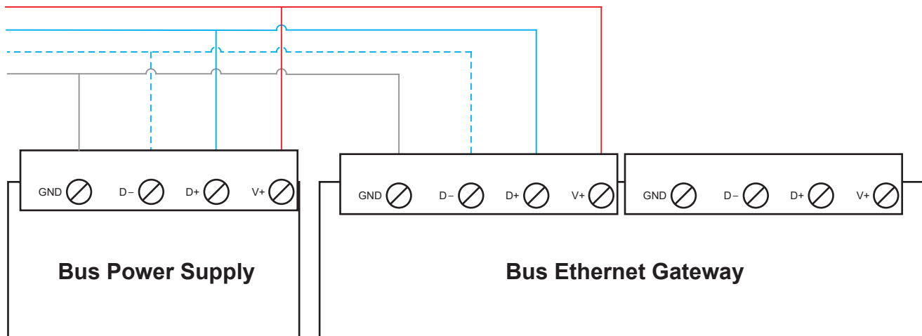
Figure 4: Bus Power Supply wiring diagram
