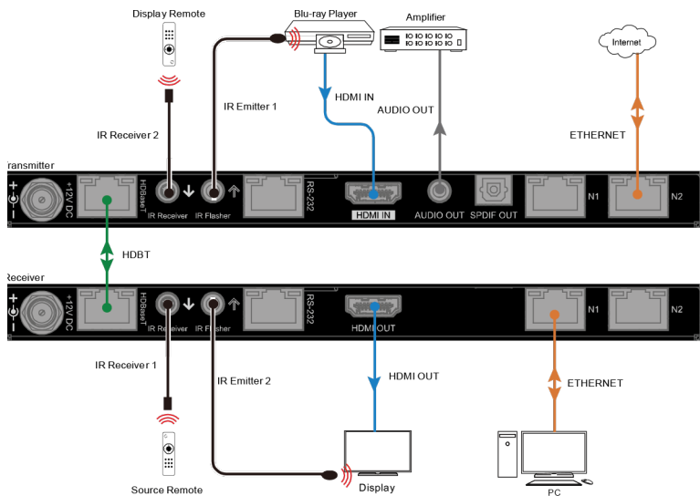
Application Diagram 1
