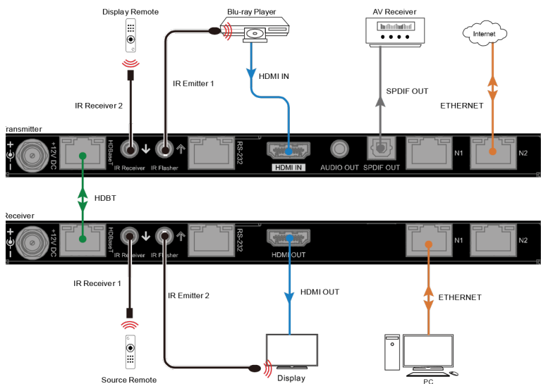
Application Diagram 2
