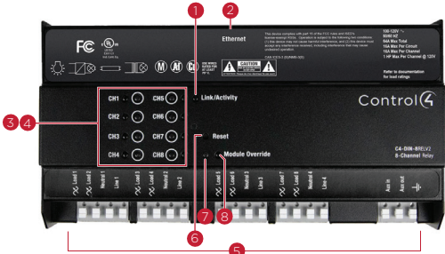
Figure 1. Front view
