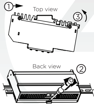
Figure 3. Attach the 8-Channel Relay Switch to a Control4 Panel
