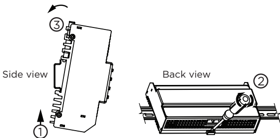
Figure 4. Attach the 8-Channel Relay Switch - third-party panels
