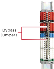
Figure 2. Terminal block bypass jumpers
